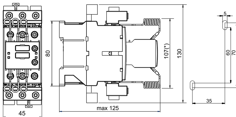
CEM 30CK
