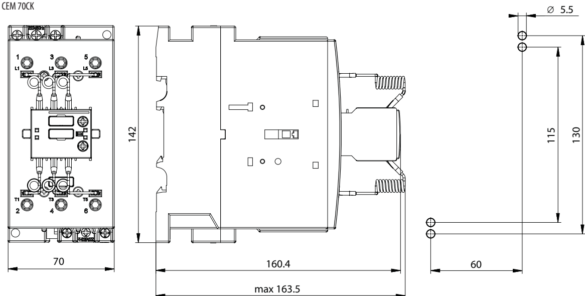
CEM 70CK
