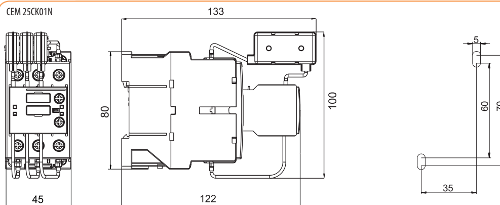
CEM 25CK01N
